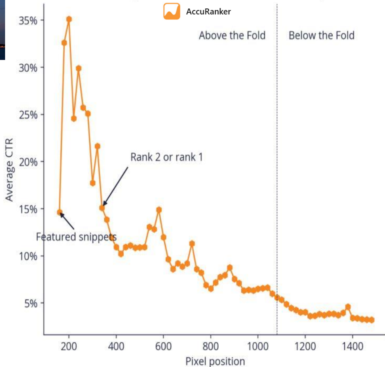
Average CTRs by pixel position (desktop)
